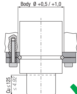
Installation with collar mount flange in upside down position.
