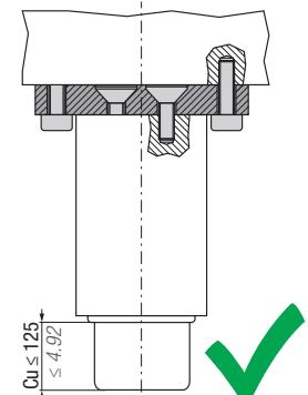
Installation with base flange through fixing screws in upside down position.
