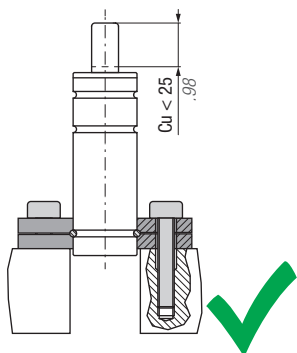
Installation with collar flange on the lower body groove.
